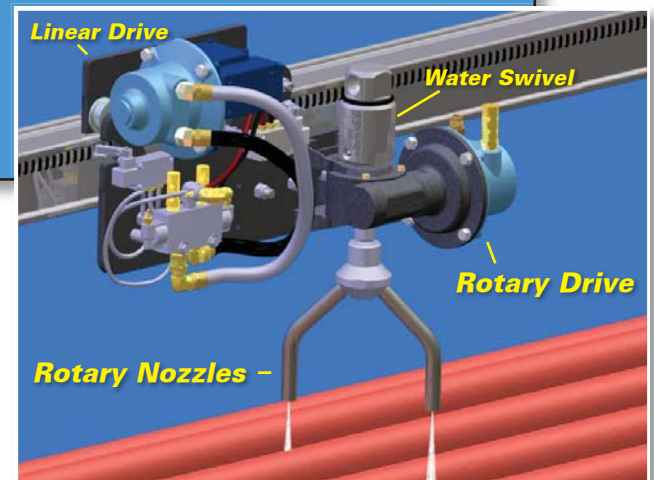
Detail of the Blastrack rotating spray head.
