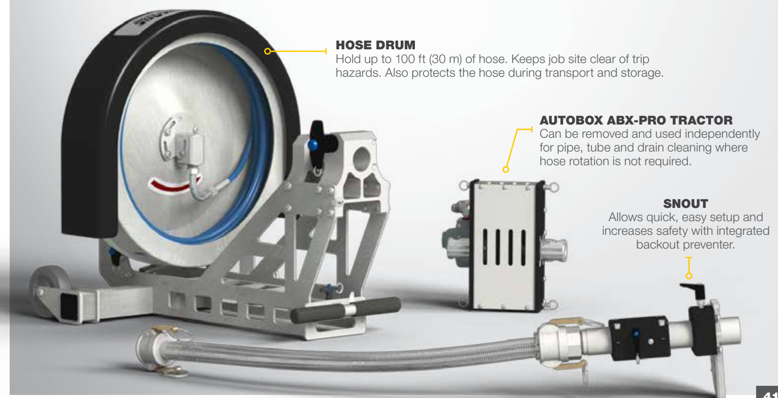
ACCOMMODATES SEVERAL HOSE SIZES Designed to work with 3/4, 1/2, and 1/4 hoses. NOTE: 4 wrap hoses are required due to hose rotation demands.
