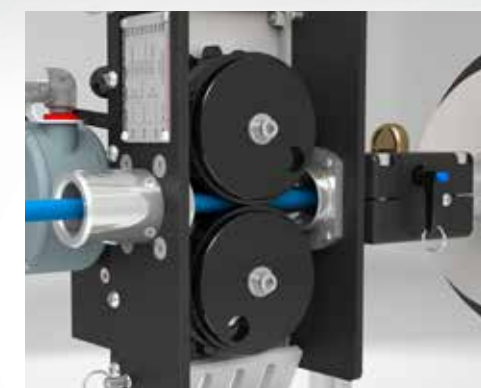
ACCOMMODATES SEVERAL HOSE SIZES Designed to work with 3/4, 1/2, and 1/4 hoses. NOTE: 4 wrap hoses are required due to hose rotation demands.
