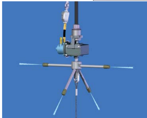
THE SM-Air CLEANING A LARGE DIAMETER STACK WITH OPTIONAL EXTENSION ARMS
