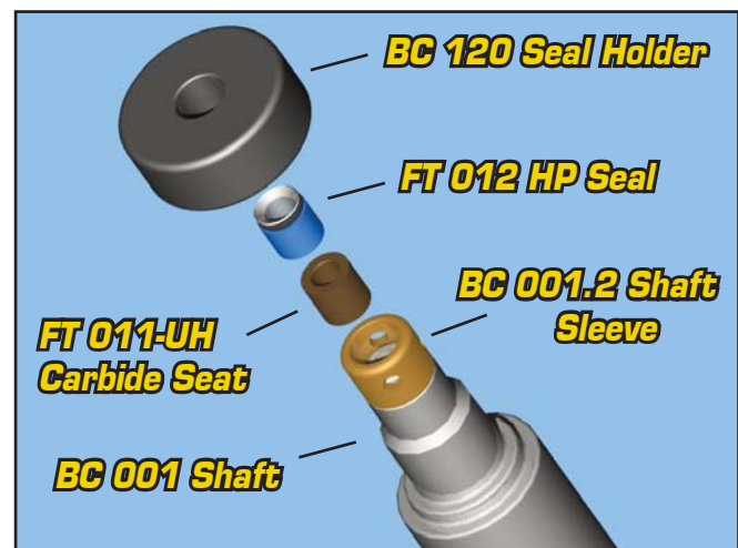
Barracuda HIGH PRESSURE SEAL ASSEMBLY
