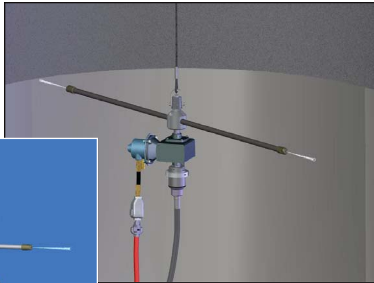
THE SM-Air CLEANING A LARGE DIAMETER STACK WITH OPTIONAL EXTENSION ARMS
