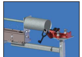
ADJUSTABLE PIPE VISE FOR 2" UP TO 5.5"
